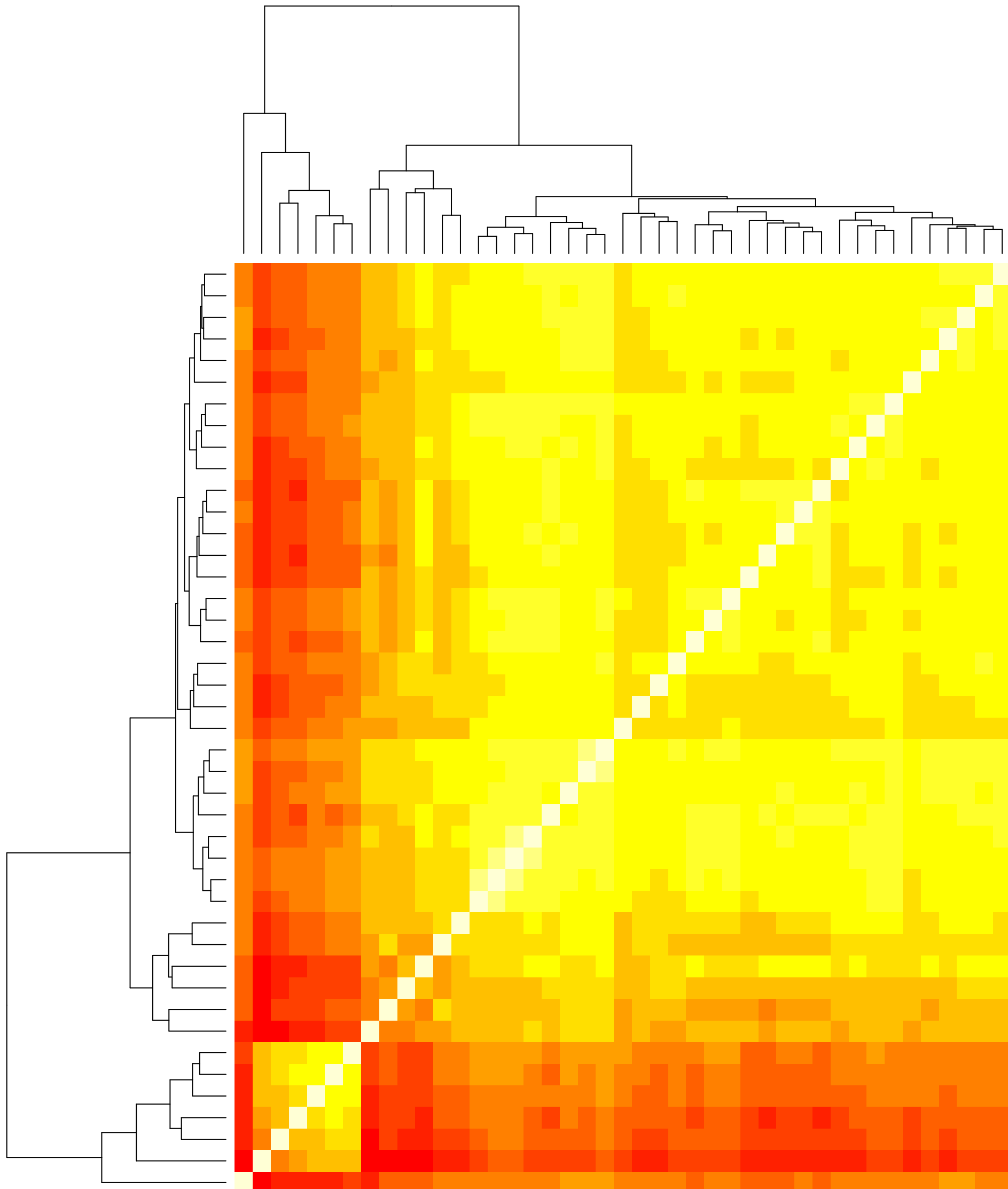
Clustering by samples for: BonaFide_CGI (yellow: high, red: low)
