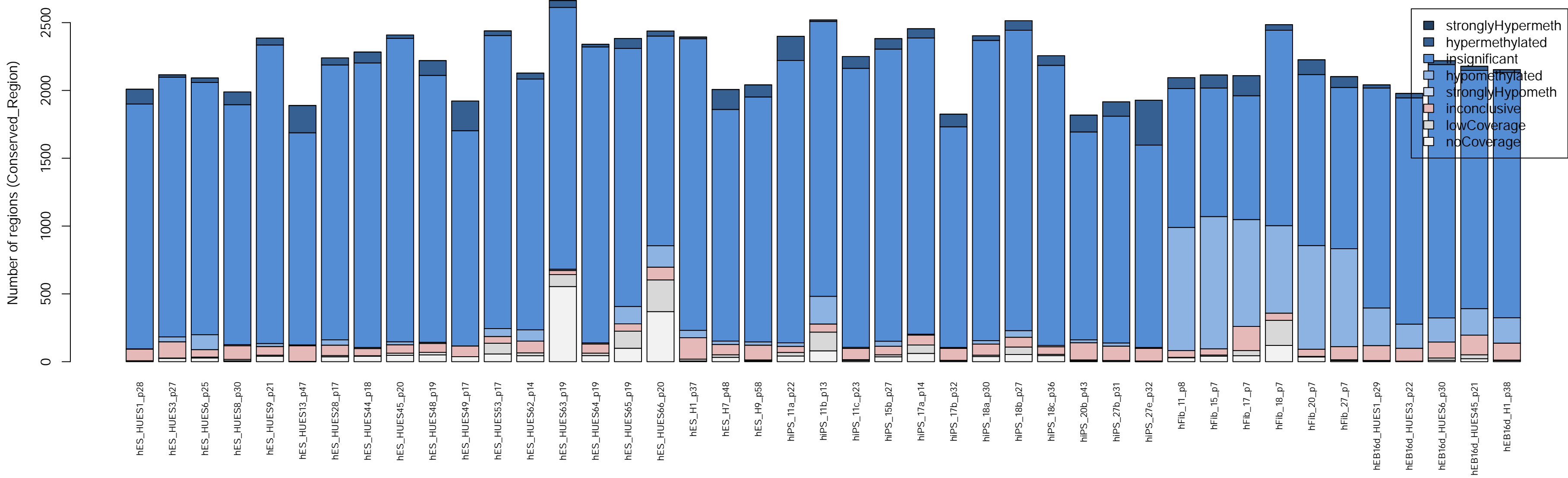
P-value based RRBS differences vs. all other regions for: Conserved_Region (#regions: 3181)
