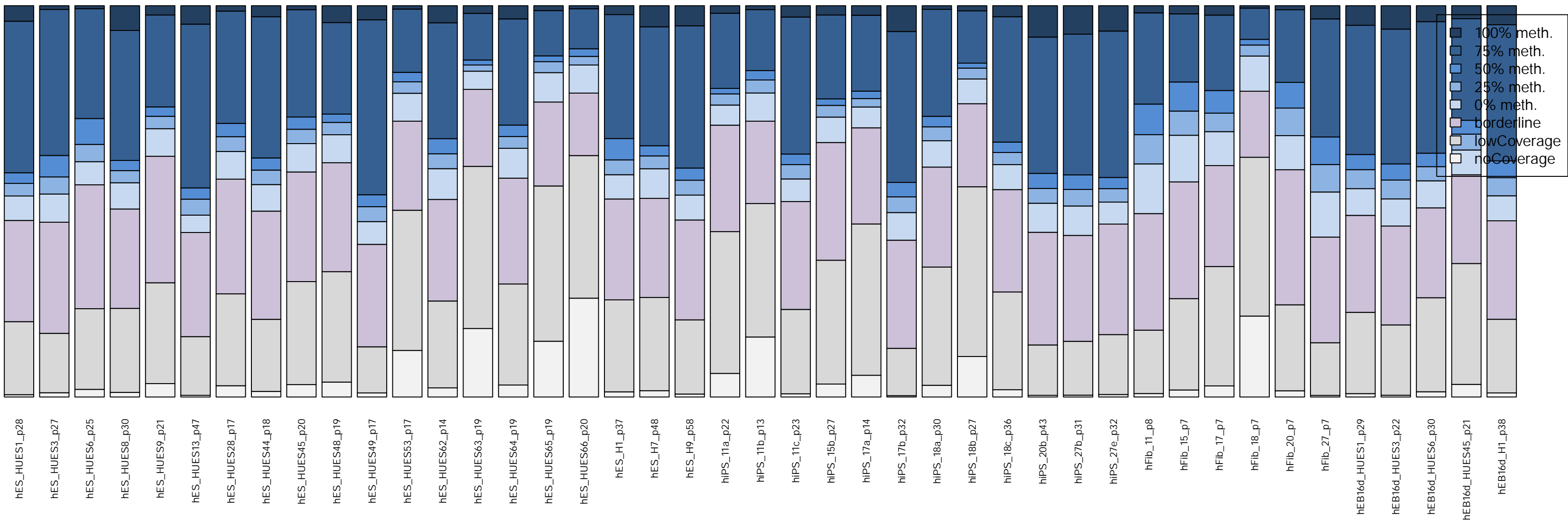
Detailed RRBS classifications for region: Enhancer_H3K4me2 (#regions: 4415)
