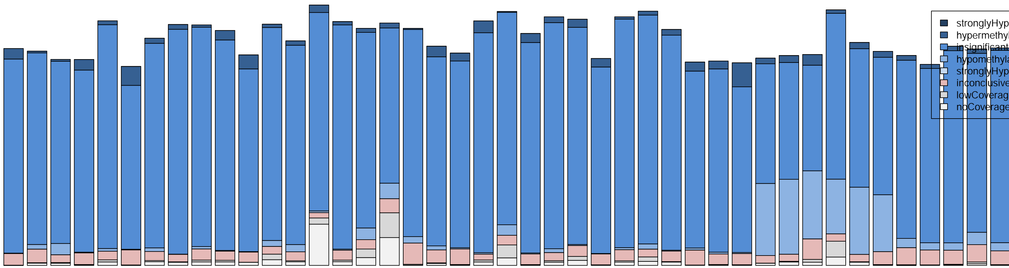
P-value based RRBS differences vs. all other regions for: Enhancer_H3K4me2 (#regions: 4415)
