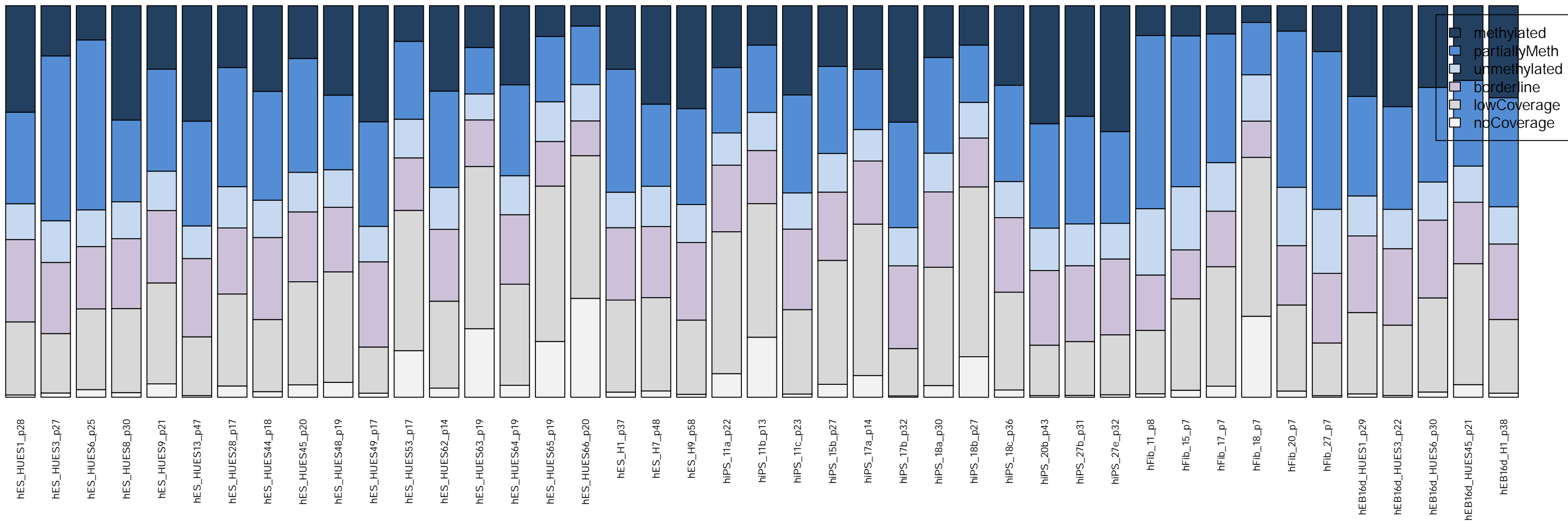
Broad RRBS classifications for region: Enhancer_H3K4me2 (#regions: 4415)
