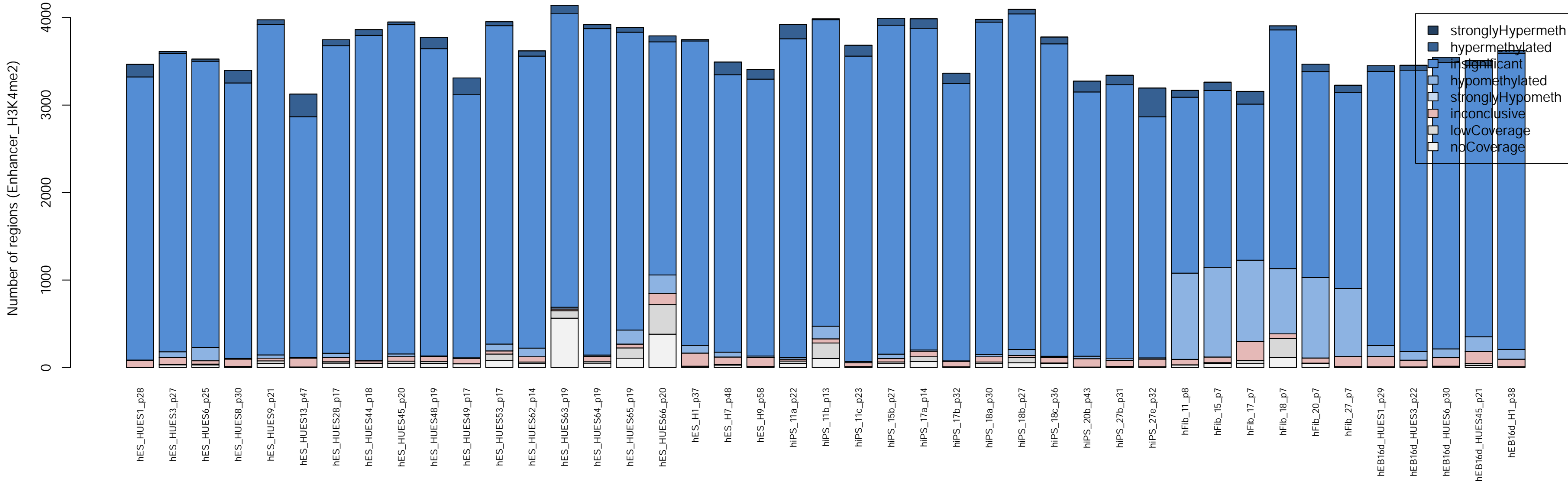
Q-value based RRBS differences vs. all other regions for: Enhancer_H3K4me2 (#regions: 4415)
