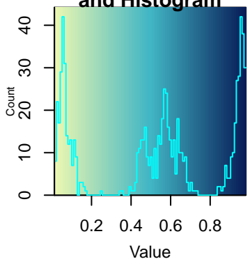
Color Key and Histogram
